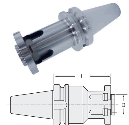
BST Boring Cutter Toolholder
