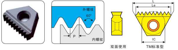
ISO标准型螺纹铣刀片 ISO Metric Full Profile
