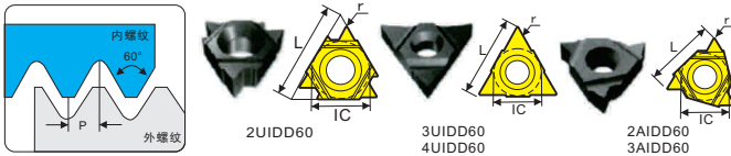
60°深孔加工螺纹铣刀片 Thread Mill for Deep Holes
