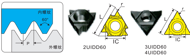
60°深孔加工螺纹铣刀片 Thread Mill for Deep Holes
