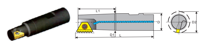
螺纹铣刀杆 Threading Milling Tool Holders
