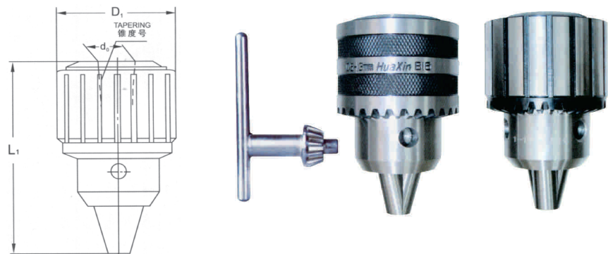
J21 SERIES TYPE L MORSE JACQUARD SHORT TAPER STOCK J21 系列 H型莫氏.贾格短锥连接
